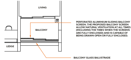
BALCONY SCREEN - PLAN
